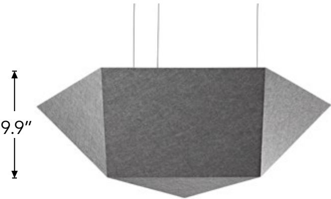
Convex Cloud Side View
