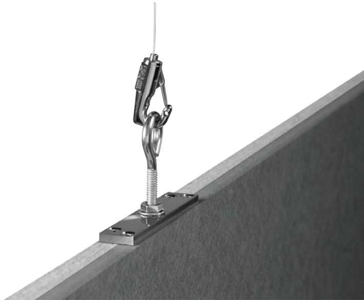
1/4"-20 Male Threaded Screw Mounting Hardware
