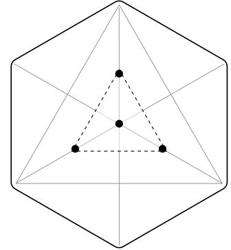
Cable Hanging Detail: Mark the centerpoint. Then measure out 7.25" out from center in an equilateral triangle shape to locate cable hanging positions.
