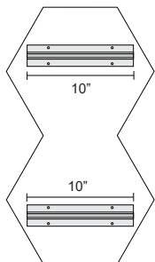
2-Diamond Cluster
