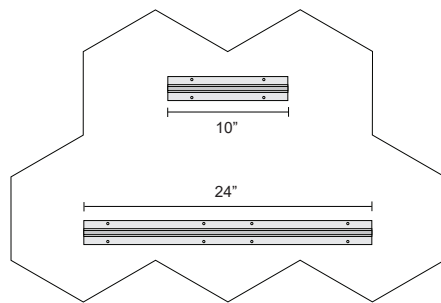
5-Diamond Cluster
