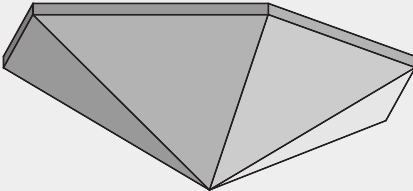
Single Diamond
