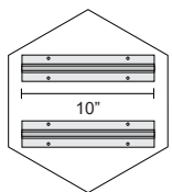
Single Diamond
